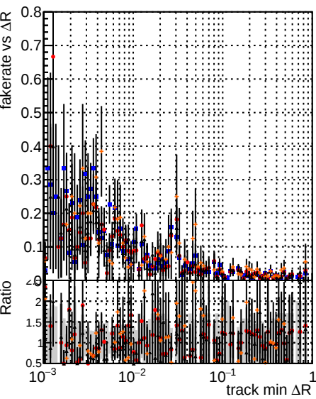
Fake rate vs \Delta R(\text{track, jet}) DQM V00001 R00000000001 Global mkFit baseline Global mkFit var Global mkFit coreNoClean Global mkFit core50maxCand-24DUPremoval
