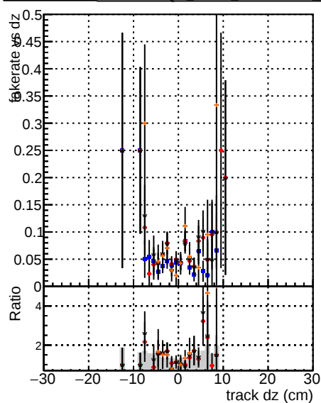
Fake rate vs dz Legend: DQM V00001, GlobalFit baseline, GlobalFit var, GlobalFit core50maxCand-24DUPremoval
