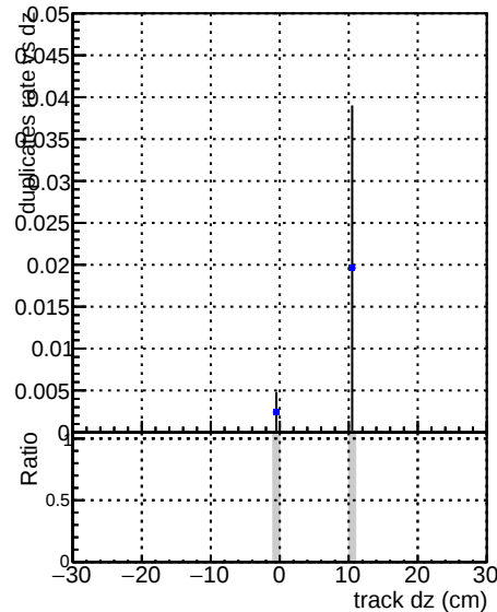
CoreNoClean core50maxCand-24DUPremoval
