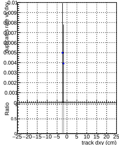
CoreNoClean core50maxCand-24DUPremoval
