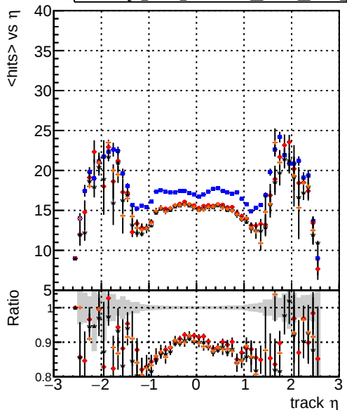
mean hits > \eta Legend: DQM_V0001_R000000001_Global_mkFit_baseline (blue), DQM_V0001_R000000001_Global_mkFit_var (red), DQM_V0001_R000000001_Global_mkFit_jcoreNoClean (black), DQM_V0001_R000000001_Global_mkFit_jcore50maxCand-24DUPremoval (orange)
