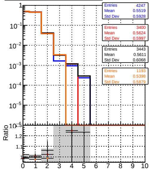
mean hits vs \eta Legend: - DQM_V0001_R000000001_Global_mkFit_baseline (blue line) - DQM_V0001_R000000001_Global_mkFit_var (red line) - DQM_V0001_R000000001_Global_mkFit_coreNoClean (black line) - DQM_V0001_R000000001_Global_mkFit_core50maxCand-24DUPremoval (orange line)
