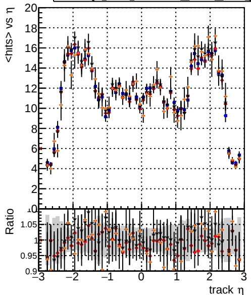
mean hits vs \eta Legend: - DQM_V0001_R000000001_Global_mkFit_baseline (blue line) - DQM_V0001_R000000001_Global_mkFit_var (red line) - DQM_V0001_R000000001_Global_mkFit_coreNoClean (black line) - DQM_V0001_R000000001_Global_mkFit_core50maxCand-24DUPremoval (orange line)
