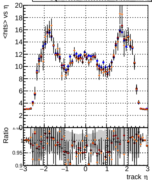
mean hits vs \eta Legend: Global mkFit baseline (blue line) Global mkFit var (red line) Global mkFit jcoreNoClean (black line) Global mkFit jcore50maxCand-24DUPremoval (orange line)
