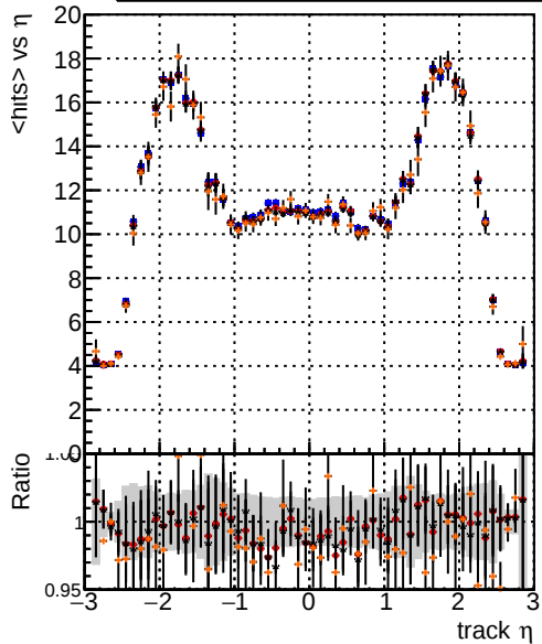
mean hits vs \eta DQM_V0001_R000000001_Global_mkFit_baseline DQM_V0001_R000000001_Global_mkFit_var DQM_V0001_R000000001_Global_mkFit_coreNoClean DQM_V0001_R000000001_Global_mkFit_core50maxCand-24DUPremoval
