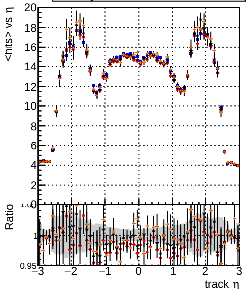
mean hits DQM_V0001_R000000001_Global_mkFit_baseline DQM_V0001_R000000001_Global_mkFit_var DQM_V0001_R000000001_Global_mkFit_coreNoClean DQM_V0001_R000000001_Global_mkFit_core50maxCand-24DUPremoval
