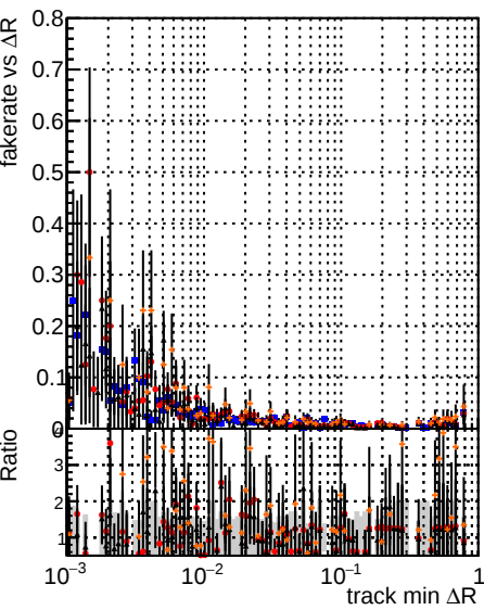
Fake rate vs \Delta R(\text{track, jet}) DQM V00001 R00000000001 Global mkFit baseline DQM V00001 R00000000001 Global mkFit var DQM V00001 R00000000001 Global mkFit coreNoClean DQM V00001 R00000000001 Global mkFit core50maxCand-24DUPremoval
