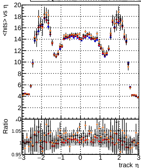
mean hit DQM_V0001_R000000001 Global mkFit baseline DQM_V0001_R000000001 Global mkFit var DQM_V0001_R000000001 Global mkFit jcoreNoClean DQM_V0001_R000000001 Global mkFit jcore50maxCand-24DUPremoval
