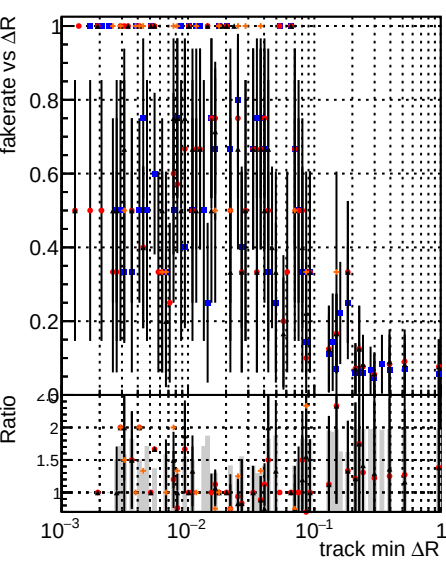
Fake rate vs \Delta R(\text{track, jet}) DQM V0001 R0000000001 Global mkFit baseline Global mkFit var Global mkFit coreNoClean Global mkFit core50maxCand-24DUPremoval
