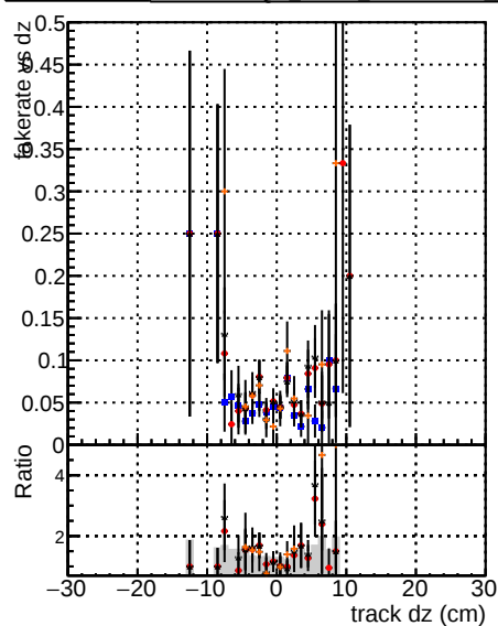
Fake rate vs dz Legend: Global, GlobalFit, GlobalFit var, GlobalFit core50max, GlobalFit core50maxCand-24DUPremoval
