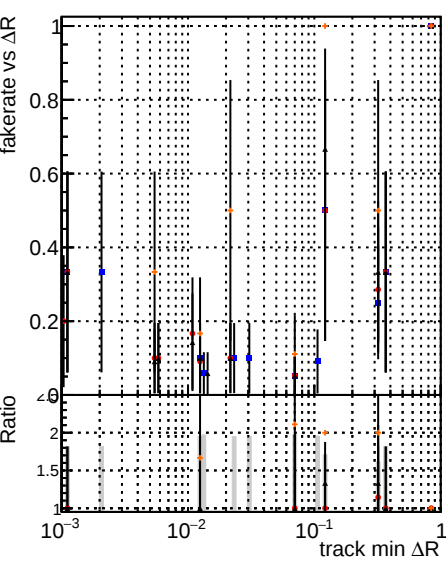
Fake rate vs \Delta R(\text{track, jet}) DQM V00001 R000000000001 Global mkFit baseline Global mkFit var Global mkFit coreNoClean Global mkFit core50maxCand-24DUPremoval
