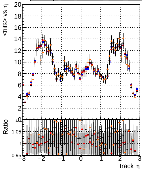
mean hit DQM_V0001_R000000001 Global mkFit baseline DQM_V0001_R000000001 Global mkFit var DQM_V0001_R000000001 Global mkFit jcoreNoClean DQM_V0001_R000000001 Global mkFit jcore50maxCand-24DUPremoval
