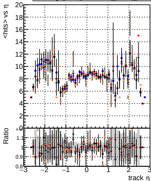
mean hits vs \eta Legend: Blue line: DQM_V0001_R000000001_Global_mkFit_baseline Red line: DQM_V0001_R000000001_Global_mkFit_var Black line: DQM_V0001_R000000001_Global_mkFit_coreNoClean Orange line: DQM_V0001_R000000001_Global_mkFit_core50maxCand-24DUPremoval
