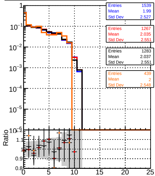
mean hits vs \eta Legend: Blue line: DQM_V0001_R000000001_Global_mkFit_baseline Red line: DQM_V0001_R000000001_Global_mkFit_var Black line: DQM_V0001_R000000001_Global_mkFit_coreNoClean Orange line: DQM_V0001_R000000001_Global_mkFit_core50maxCand-24DUPremoval
