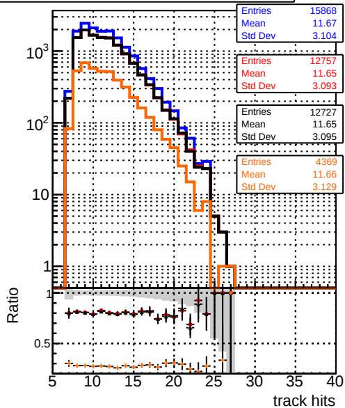
mean hits Legend: DQM_V0001_R000000001_Global_mkFit_baseline DQM_V0001_R000000001_Global_mkFit_var DQM_V0001_R000000001_Global_mkFit_coreNoClean DQM_V0001_R000000001_Global_mkFit_core50maxCand-24DUPremoval
