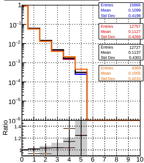
mean hits Legend: DQM_V0001_R000000001_Global_mkFit_baseline DQM_V0001_R000000001_Global_mkFit_var DQM_V0001_R000000001_Global_mkFit_coreNoClean DQM_V0001_R000000001_Global_mkFit_core50maxCand-24DUPremoval
