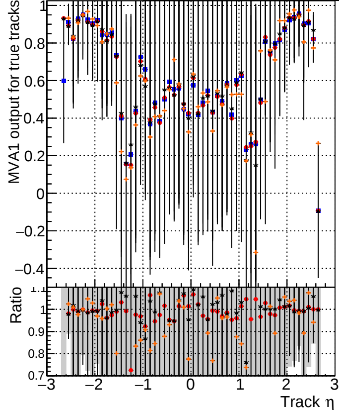
MVA1 of associated tracks (recoToSim) vs. track \eta Legend: DQM_V0001_R0000000001_Global_mkFit_baseline (blue square) DQM_V0001_R0000000001_Global_mkFit_var (red circle) DQM_V0001_R0000000001_Global_mkFit_coreNoClean (black triangle) DQM_V0001_R0000000001_Global_mkFit_core50maxCand-24DUPremoval (orange cross)
