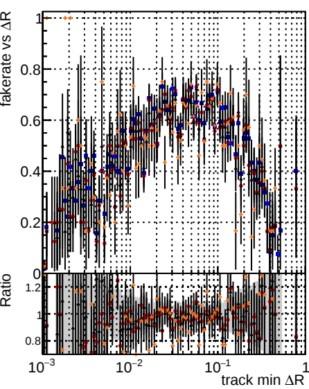
Fake rate vs \Delta R (track, jet) | Duplicates Rate vs \Delta R (track, jet) | Pileup rate vs \Delta R (track, jet) Legend: DQM (black), V0001 (blue), R0000000001 (orange), Global (grey), mkFit (green), baseline (red), var (purple), coreNoClean (brown), core50maxCand-24DUPremoval (pink).
