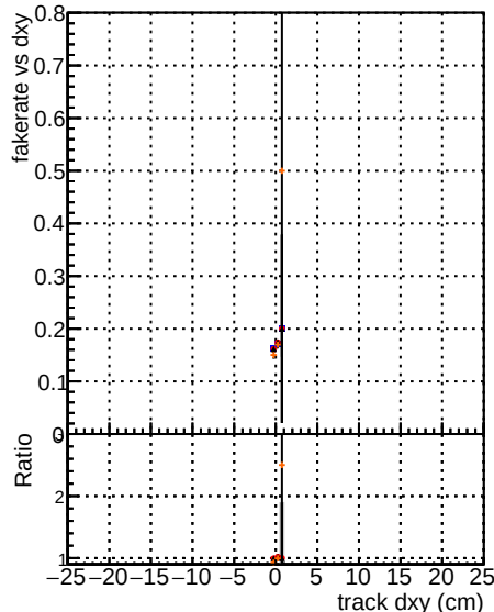
Fake rate vs d DGM V00001 D00000000001 Global mkFit baseline DGM V00001 R00000000001 Global mkFit coreNoClean DGM V00001 R00000000001 Global mkFit core50maxCand-24DUPremoval
