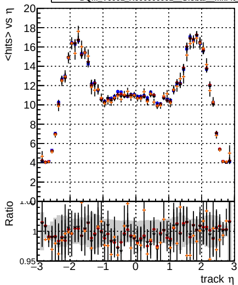
mean hits vs \eta Legend: DQM_V0001_R000000001_Global_mkFit_baseline DQM_V0001_R000000001_Global_mkFit_var DQM_V0001_R000000001_Global_mkFit_coreNoClean DQM_V0001_R000000001_Global_mkFit_core50maxCand-24DUPremoval
