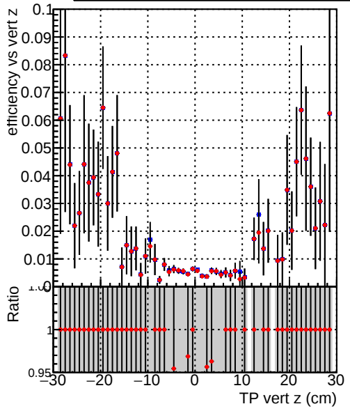
Efficiency vs vertpos Legend: DQM_V0001_R0000000001_Global_mkFit_baseline DQM_V0001_R0000000001_Global_mkFit_core50maxCand-24DUPremoval-1000
