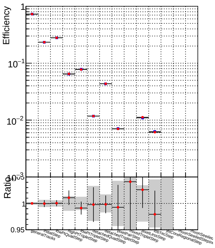
DQM_V0001_R000000001_Global_mkFit_baseline DQM_V0001_R000000001_Global_mkFit_jcore50maxCand-24DUPremoval-1000
