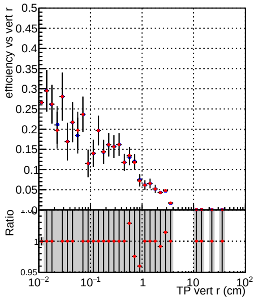
Efficiency vs vertpos Legend: DQM_V0001_R000000001_Global_mkFit_baseline DQM_V0001_R000000001_Global_mkFit_core50maxCand-24DUPremoval-1000
