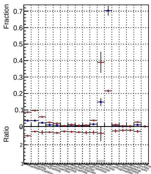
— DQM_V0001_R000000001_Global_mkFit_baseline — DQM_V0001_R000000001_Global_mkFit_core50maxCand-24DUPremoval-1000
