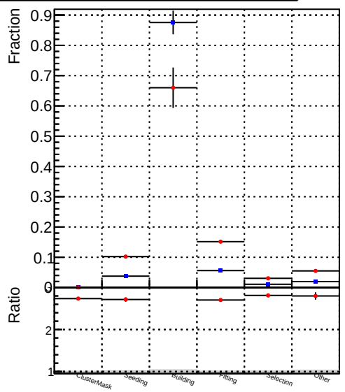
— DQM_V0001_R000000001_Global_mkFit_baseline — DQM_V0001_R000000001_Global_mkFit_core50maxCand-24DUPremoval-1000
