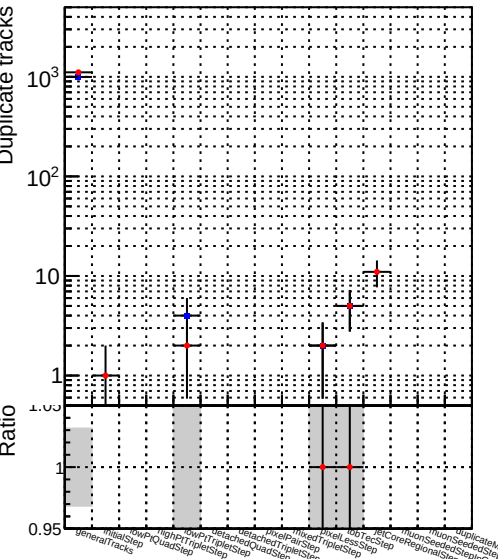
Number DQM_V0001_R000000001_Global_mkFit_jcore50maxCand-24DUPremoval-1000
