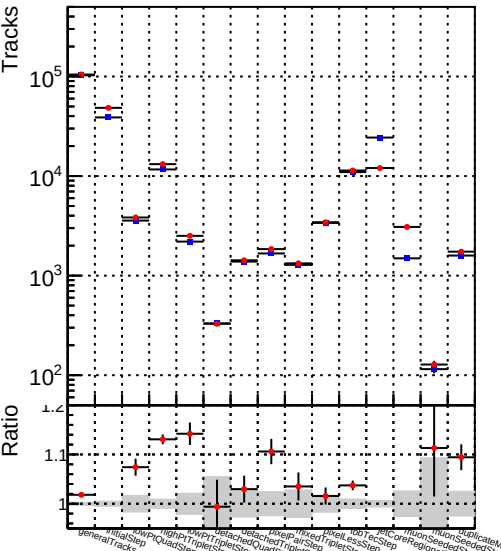
DQM_V0001_R000000001_Global_mkFit_baseline
