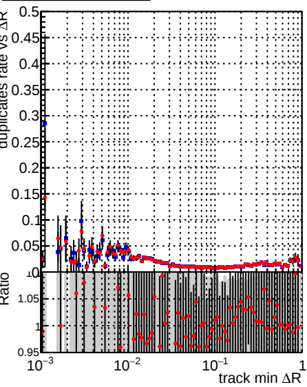
Legend: - Blue dots with error bars: DQM_V0001_R000000001_Global_mkFit_baseline - Red dots with error bars: DQM_V0001_R000000001_Global_mkFit_jcore50maxCand-24DUPremoval-1000
