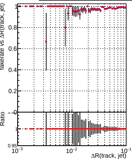
Legend: - Blue dots with error bars: DQM_V0001_R000000001_Global_mkFit_baseline - Red dots with error bars: DQM_V0001_R000000001_Global_mkFit_jcore50maxCand-24DUPremoval-1000
