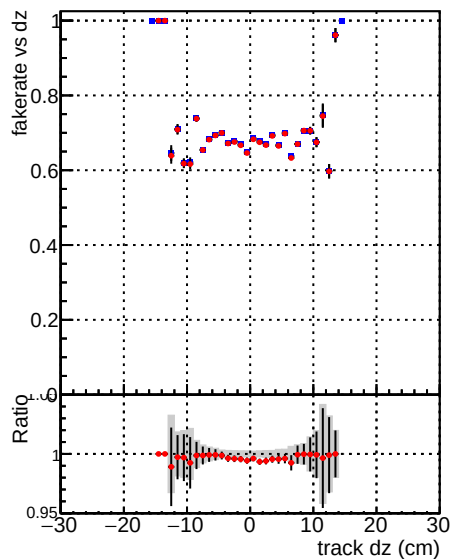
Fake rate vs dz DQM V0001_R000000001 Global mkFit baseline DQM V0001_R000000001 Global mkFit_jcore50maxCand-24DUPremoval-1000
