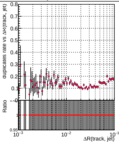
—●— DQM_V0001_R000000001_Global_mkFit_baseline —●— DQM_V0001_R000000001_Global_mkFit_jcore50maxCand-24DUPremoval-1000
