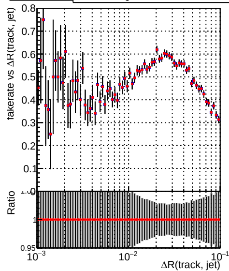
—●— DQM_V0001_R000000001_Global_mkFit_baseline —●— DQM_V0001_R000000001_Global_mkFit_jcore50maxCand-24DUPremoval-1000
