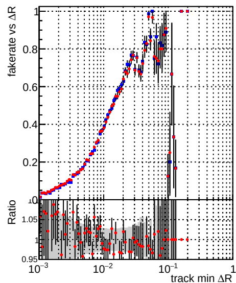
—●— DQM_V0001_R000000001_Global_mkFit_baseline —●— DQM_V0001_R000000001_Global_mkFit_jcore50maxCand-24DUPremoval-1000
