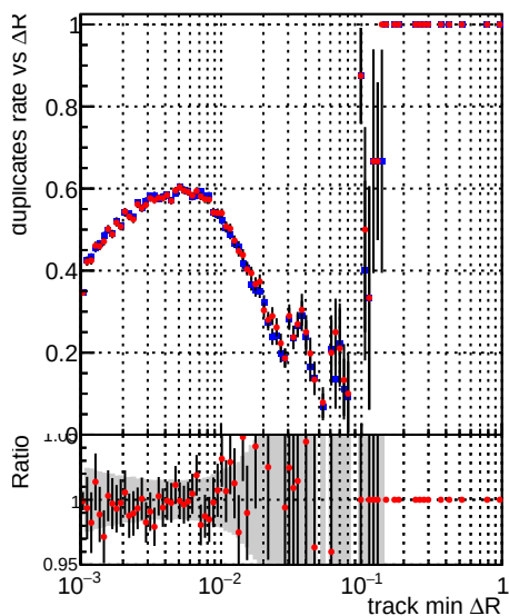
—●— DQM_V0001_R000000001_Global_mkFit_baseline —●— DQM_V0001_R000000001_Global_mkFit_jcore50maxCand-24DUPremoval-1000
