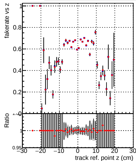
—●— DQM_V0001_R000000001_Global_mkFit_baseline —●— DQM_V0001_R000000001_Global_mkFit_jcore50maxCand-24DUPremoval-1000
