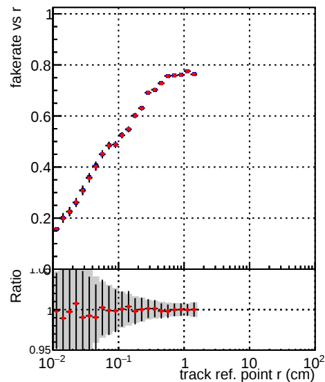
—●— DQM_V0001_R000000001_Global_mkFit_baseline —●— DQM_V0001_R000000001_Global_mkFit_jcore50maxCand-24DUPremoval-1000
