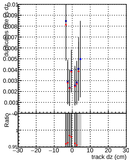
—●— DQM_V0001_R0000000001_Global_mkFit_baseline —●— DQM_V0001_R0000000001_Global_mkFit_jcore50maxCand-24DUPremoval-1000
