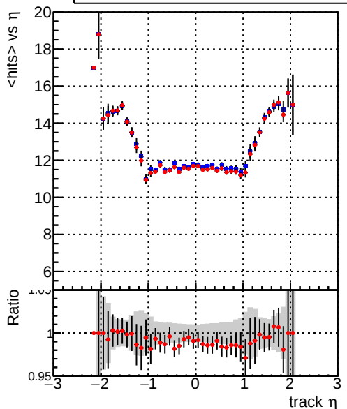
DQM_V0001_R000000001_Global_mkFit_baseline mean hit DQM_V0001_R000000001_Global_mkFit_core50maxCand-24DUPremoval-1000
