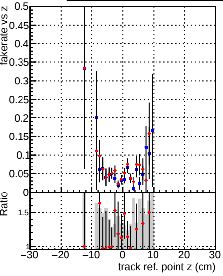
—●— DQM_V0001_R000000001_Global_mkFit_baseline —●— DQM_V0001_R000000001_Global_mkFit_jcore50maxCand-24DUPremoval-1000
