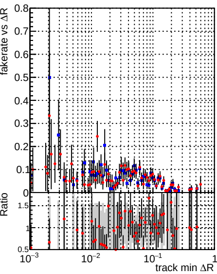
Legend: - \blacksquare DQM_V0001_R000000001_Global_mkFit_baseline - \bullet DQM_V0001_R000000001_Global_mkFit_jcore50maxCand-24DUPremoval-1000
