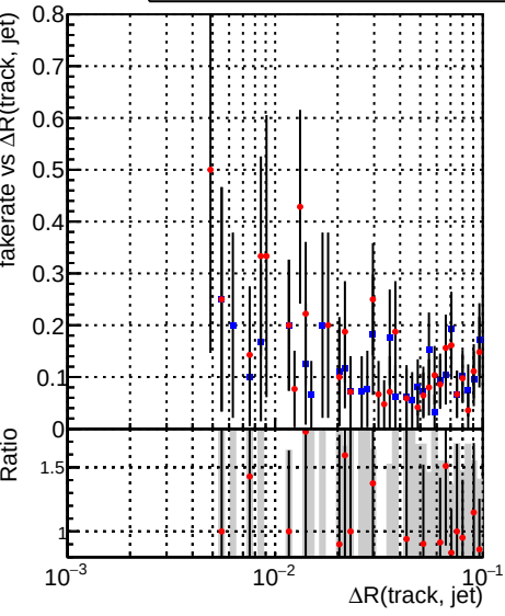
Legend: - \blacksquare DQM_V0001_R000000001_Global_mkFit_baseline - \bullet DQM_V0001_R000000001_Global_mkFit_jcore50maxCand-24DUPremoval-1000
