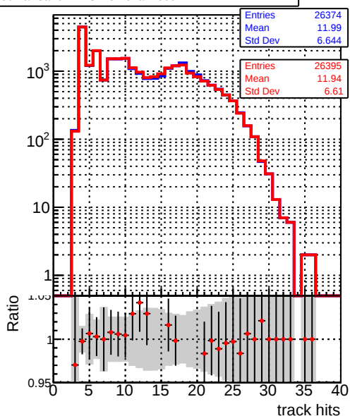
DQM_V0001_R000000001_Global_mkFit_core50maxCand-24DUPremoval-1000
