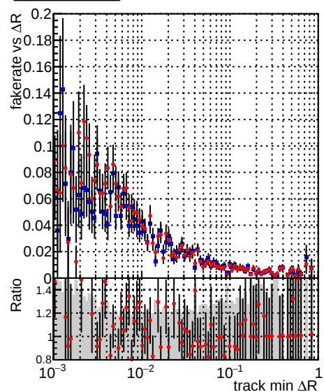
■ DQM_V0001_R000000001_Global_mkFit_baseline ● DQM_V0001_R000000001_Global_mkFit_jcore50maxCand-24DUPremoval-1000
