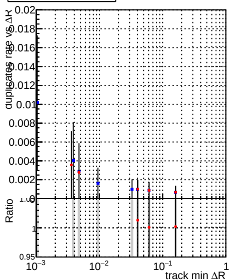
■ DQM_V0001_R000000001_Global_mkFit_baseline ● DQM_V0001_R000000001_Global_mkFit_jcore50maxCand-24DUPremoval-1000
