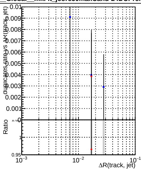
■ DQM_V0001_R000000001_Global_mkFit_baseline ● DQM_V0001_R000000001_Global_mkFit_jcore50maxCand-24DUPremoval-1000
