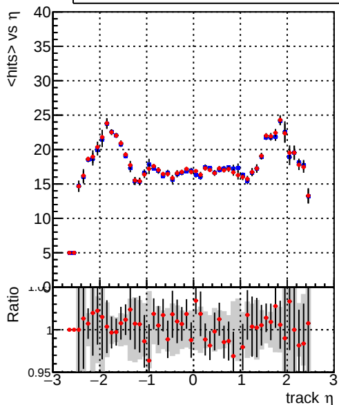
mean hits vs \eta — DQM_V0001_R000000001_Global_mkFit_baseline — DQM_V0001_R000000001_Global_mkFit_core50maxCand-24DUPremoval-1000
