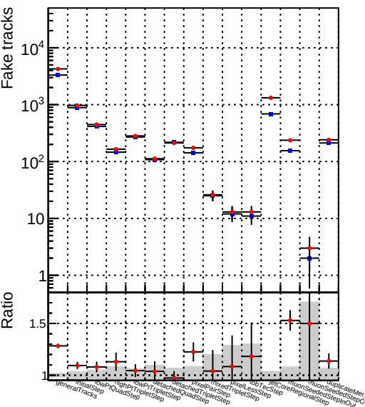
Number ● DQM_V0001_R000000001_Global_mkFit_jcore50maxCand-24DUPremoval-1000
