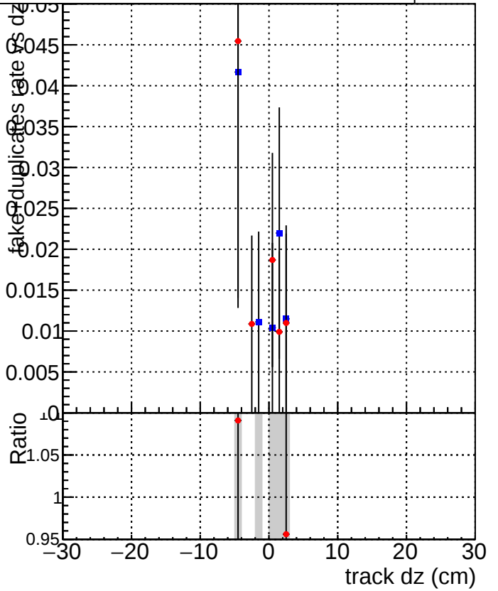
DQM_V0001_R000000001_Global_mkFit_baseline DQM_V0001_R000000001_Global_mkFit_jcore50maxCand-24DUPremoval-1000
