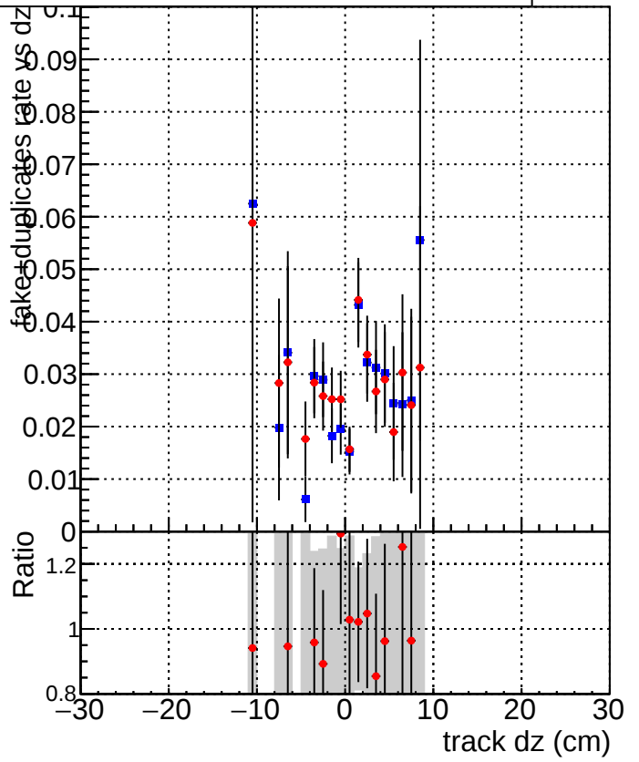
DQM_V0001_R000000001_Global_mkFit_baseline DQM_V0001_R000000001_Global_mkFit_jcore50maxCand-24DUPremoval-1000
