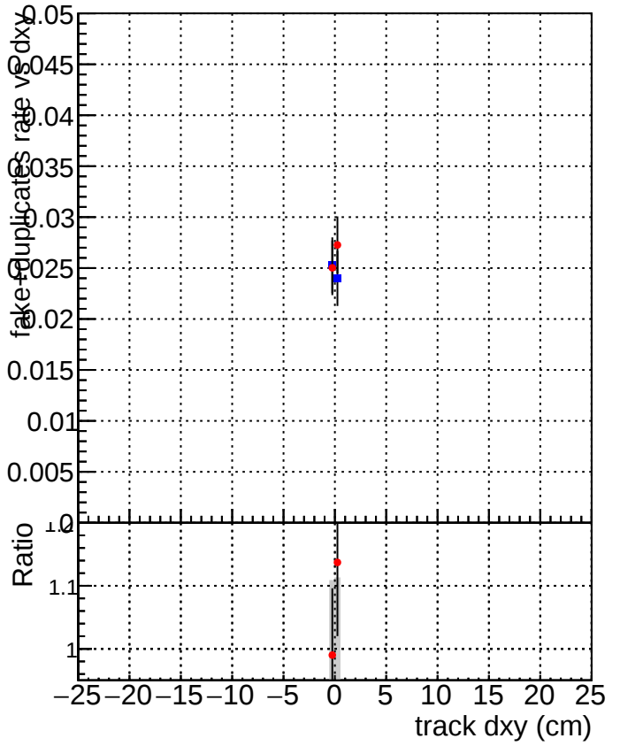
DQM_V0001_R000000001_Global_mkFit_baseline DQM_V0001_R000000001_Global_mkFit_jcore50maxCand-24DUPremoval-1000
