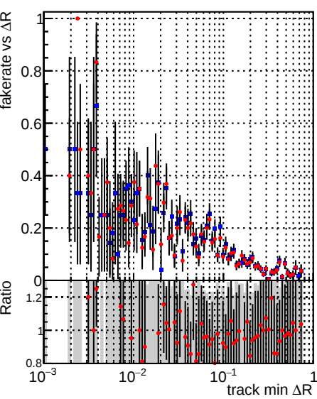
Legend: DQM_V0001_R000000001_Global_mkFit_baseline (blue squares), DQM_V0001_R000000001_Global_mkFit_jcore50maxCand-24DUPremoval-1000 (red circles)
