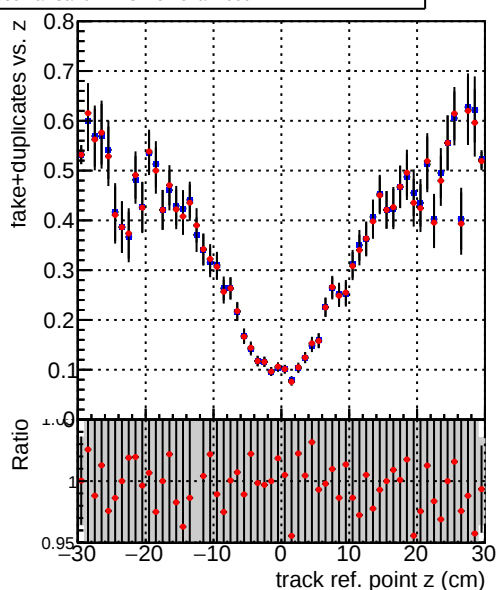
— DQM_V0001_R000000001_Global_mkFit_baseline — DQM_V0001_R000000001_Global_mkFit_core50maxCand-24DUPremoval-1000
