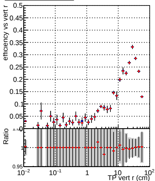
— DQM_V0001_R000000001_Global_mkFit_baseline — DQM_V0001_R000000001_Global_mkFit_core50maxCand-24DUPremoval-1000
