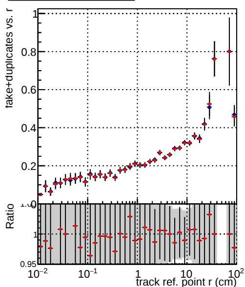
— DQM_V0001_R000000001_Global_mkFit_baseline — DQM_V0001_R000000001_Global_mkFit_core50maxCand-24DUPremoval-1000
