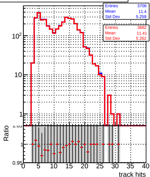
DQM_V0001_R000000001_Global_mkFit_core50maxCand-24DUPremoval-1000
