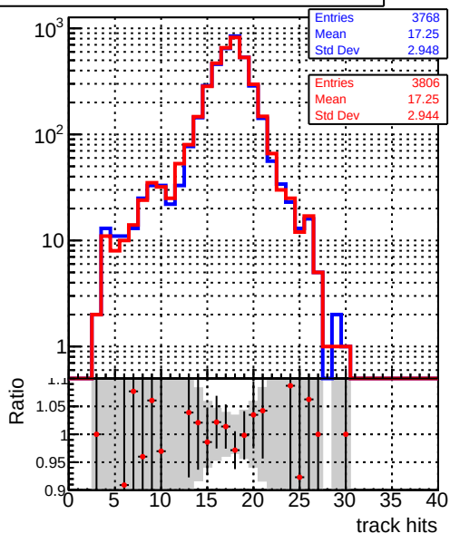
— DQM_V0001_R000000001_Global_mkFit_baseline — DQM_V0001_R000000001_Global_mkFit_core50maxCand-24DUPremoval-1000
