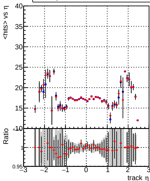
— DQM_V0001_R000000001_Global_mkFit_baseline — DQM_V0001_R000000001_Global_mkFit_core50maxCand-24DUPremoval-1000
