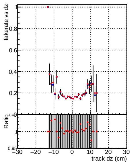
Fake rate vs dz —●— DQM_V0001_R0000000001_Global_mkFit_baseline —●— DQM_V0001_R0000000001_Global_mkFit_jcore50maxCand-24DUPremoval-1000
