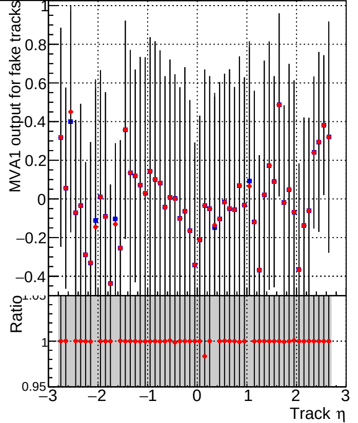
MVA1 of associated tracks (recoToSim) vs. track \eta ■ DQM_V0001_R000000001_Global_mkFit_baseline ■ DQM_V0001_R000000001_Global_mkFit_jcore50maxCand-24DUPremoval-1000
