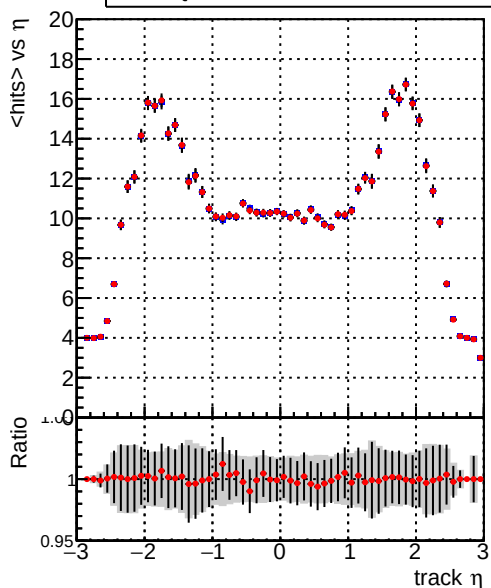
mean hit — DQM_V0001_R000000001_Global_mkFit_baseline — DQM_V0001_R000000001_Global_mkFit_core50maxCand-24DUPremoval-1000
