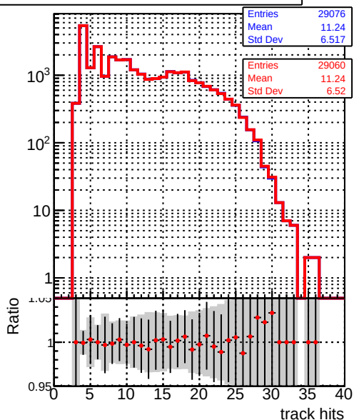
mean hit — DQM_V0001_R000000001_Global_mkFit_baseline — DQM_V0001_R000000001_Global_mkFit_core50maxCand-24DUPremoval-1000
