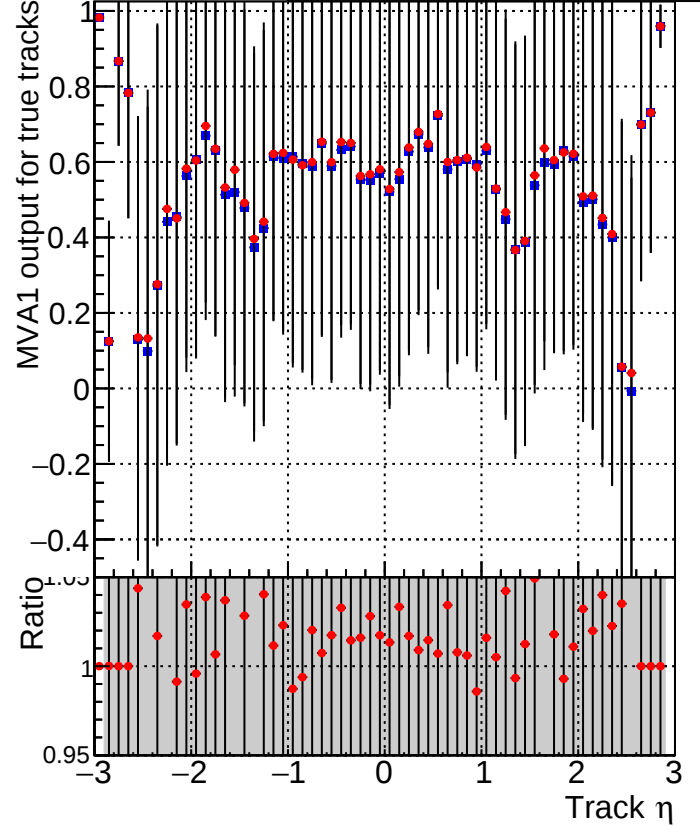
MVA1 of associated tracks (recoToSim) vs. track \eta Legend: ■ DQM_V0001_R000000001_Global_mkFit_baseline ● DQM_V0001_R000000001_Global_mkFit_jcore50maxCand-24DUPremoval-1000
