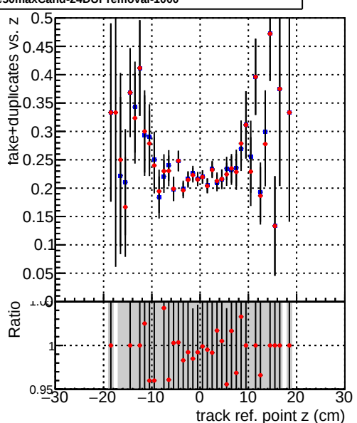
— DQM_V0001_R000000001_Global_mkFit_baseline — DQM_V0001_R000000001_Global_mkFit_core50maxCand-24DUPremoval-1000
