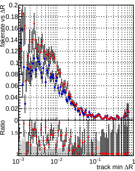
Legend: \blacksquare DQM_V0001_R000000001_Global_mkFit_baseline \blacktriangle DQM_V0001_R000000001_Global_mkFit_jcore50maxCand-24DUPremoval-1000
