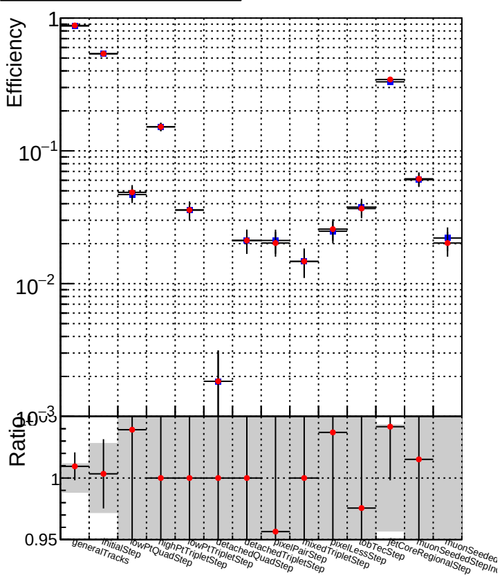
DQM_V0001_R000000001_Global_mkFit_baseline DQM_V0001_R000000001_Global_mkFit_jcore50maxCand-24DUPremoval-1000
